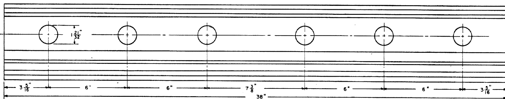
ELEVATION OF JOINT BAR
