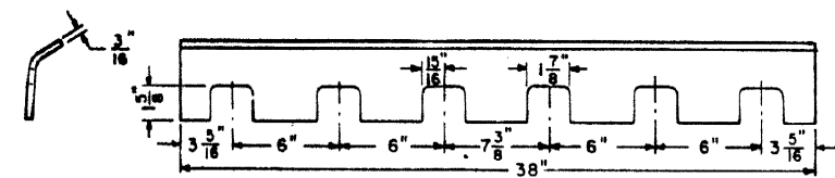
FIBRE HEAD PIECE
