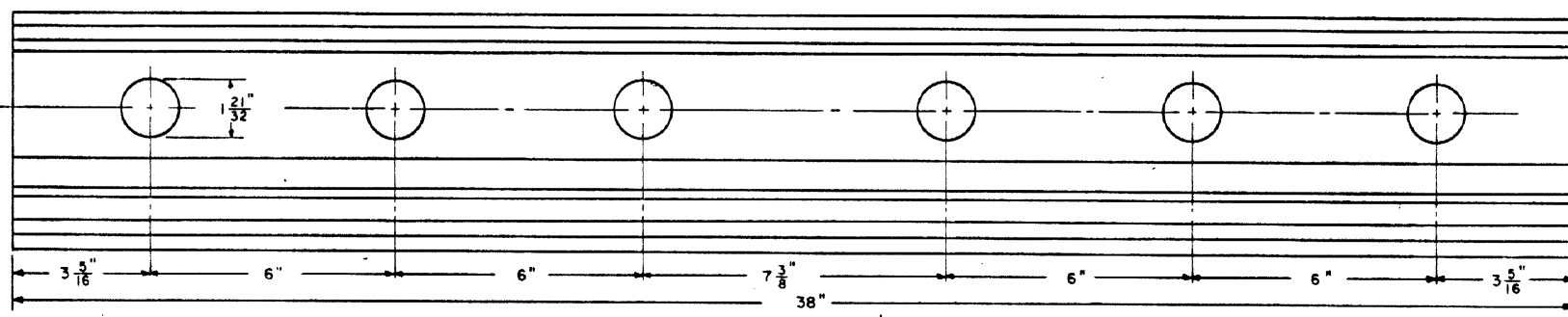
ELEVATION OF JOINT BAR
