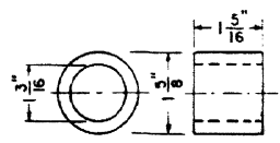
FIBRE BUSHING
