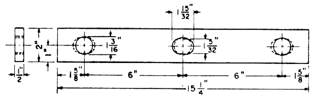
STEEL WASHER PLATE
