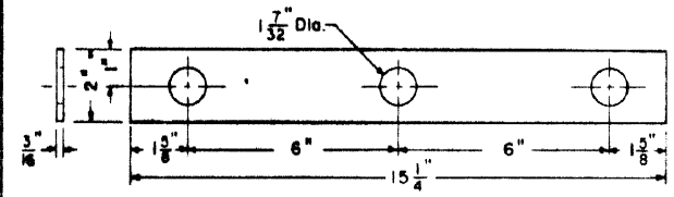
FIBRE WASHER PLATE
