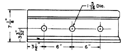
RAIL END DRILLING
