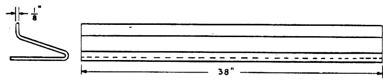
FIBRE BASE PIECE
