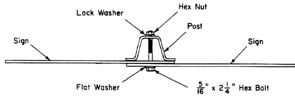
DETAIL OF MOUNTING SIGNS
