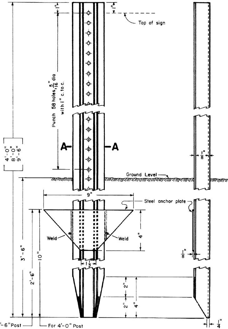
DETAIL OF POST
