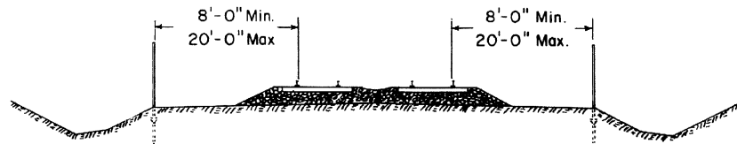
TYPICAL LOCATION OF POST
