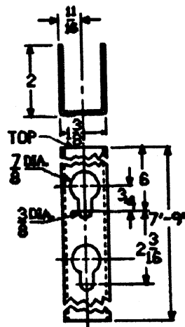
SHELF SUPPORT DETAIL MATERIAL - 11 GAGE (8.119%) MSS STEEL
