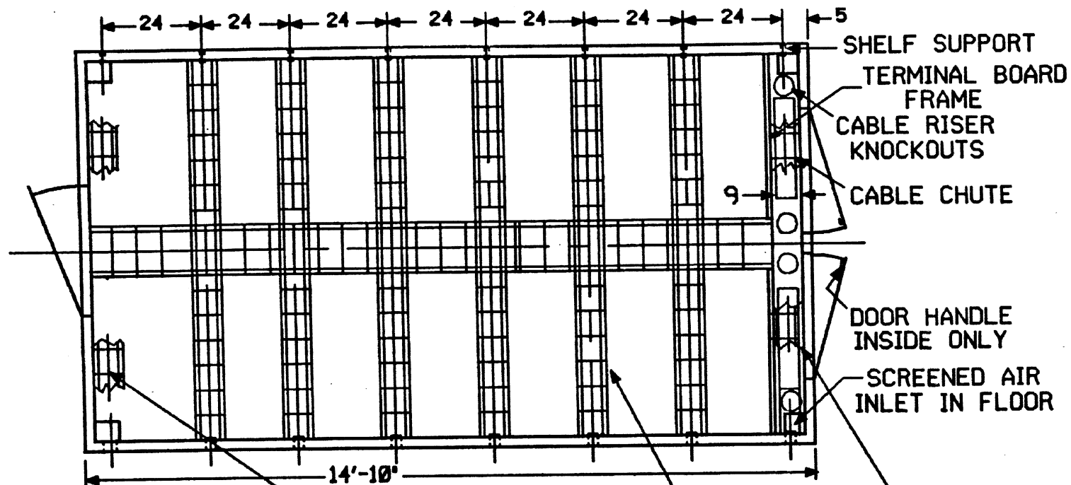
PLAN VIEW LADDER TYPE WIREWAYS
