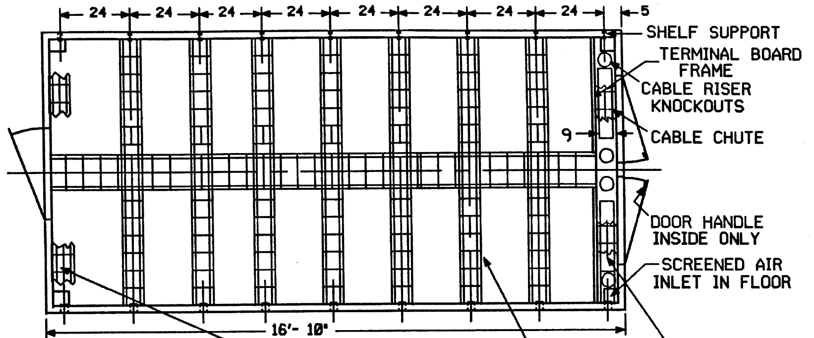
PLAN VIEW LADDER TYPE WIREWAYS
