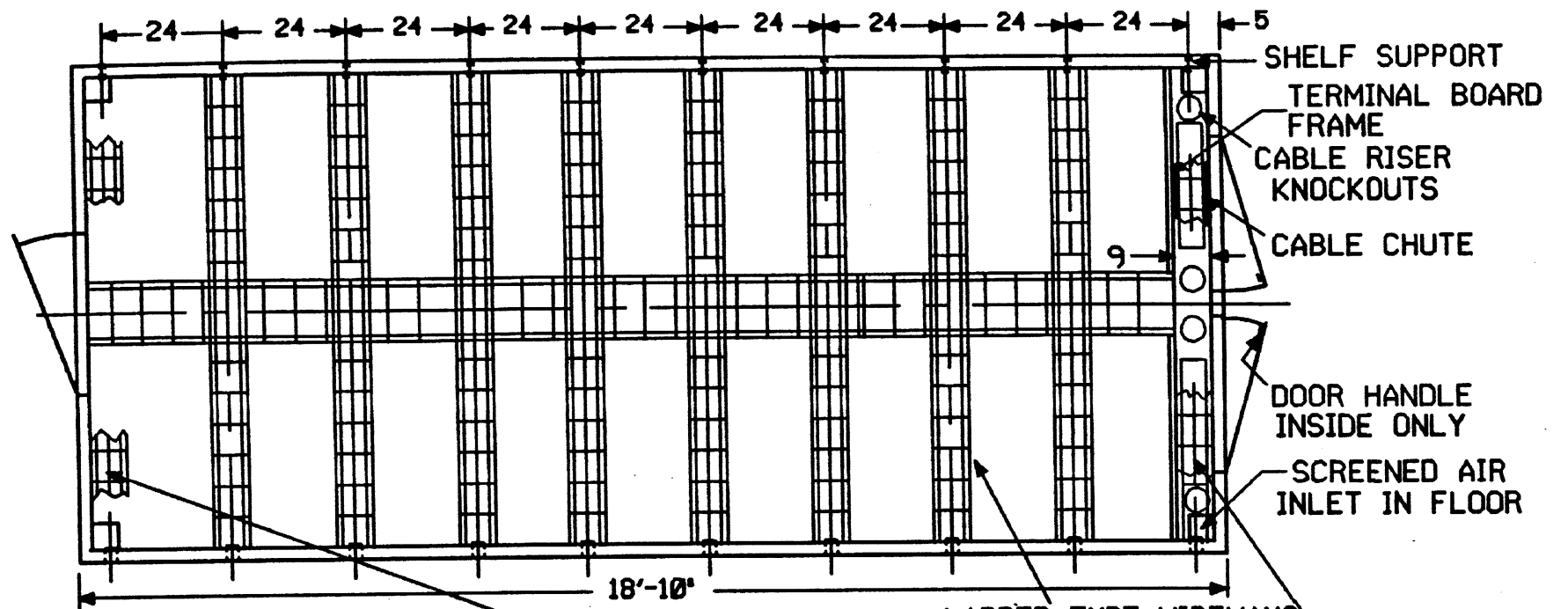
PLAN VIEW LADDER TYPE WIREWAYS
