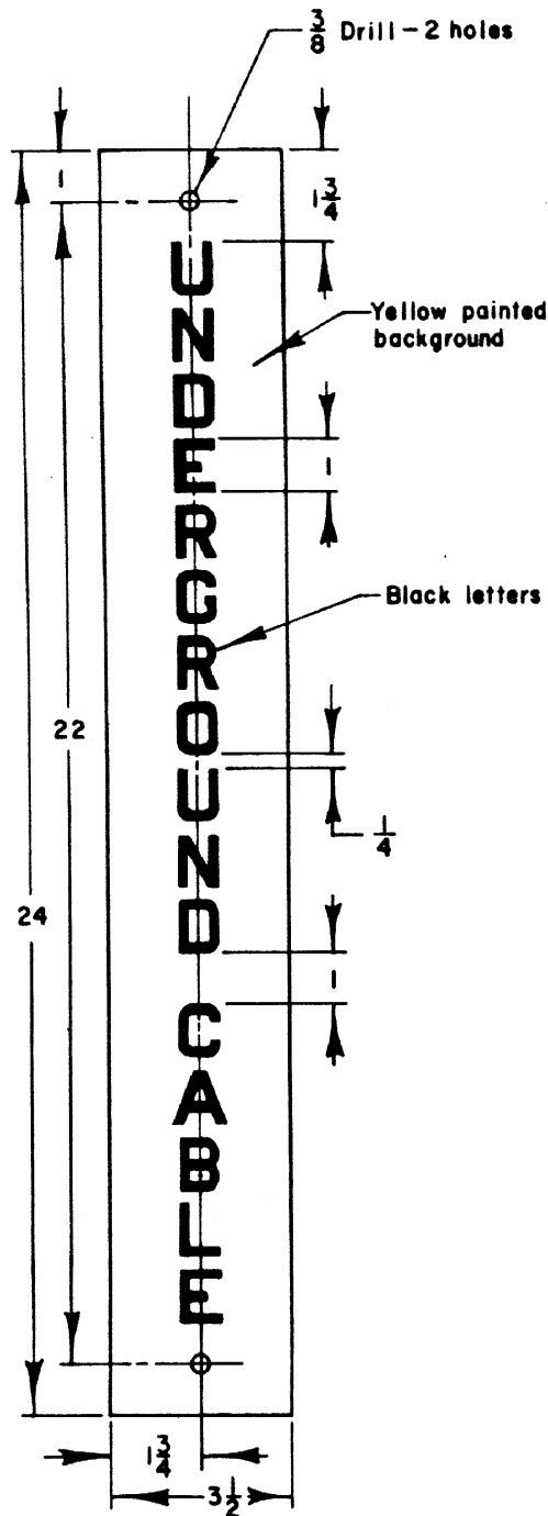
UNDERGROUND CABLE 7001-1
