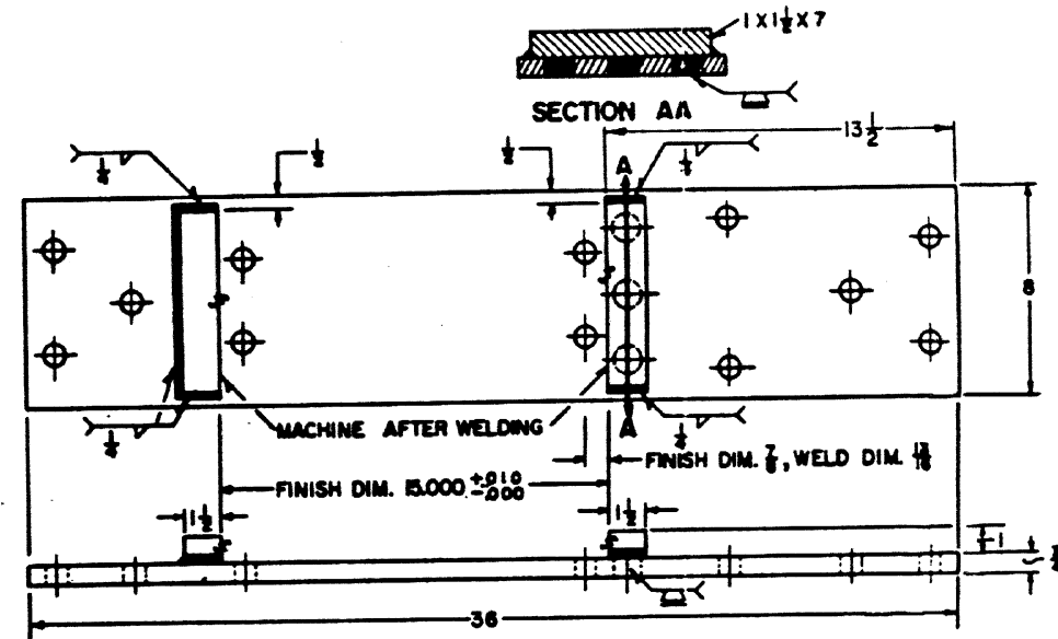
BUTT STRAP WELDING DETAIL FOR FIGS. 1, 3 & 4
