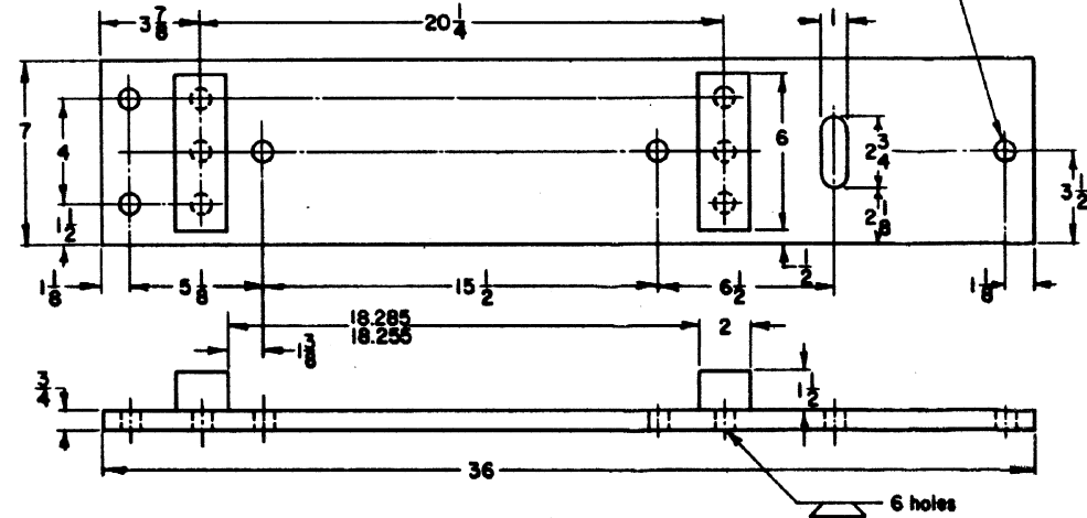
8004-17, SADDLE PLATE, G.R.S. 5F & 5H Machines
