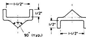
BOLT GRIP 82164 Material - 3/16" thick mild sheet steel coated per note L 02-611505
