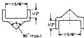
BOLT GRIP 82163 Material - 3/16" thick mild sheet steel coated per note L 02-611257
