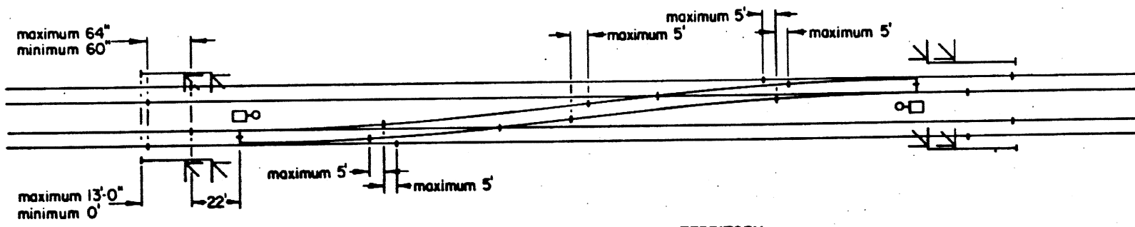
INTERLOCKED CROSSOVERS-CAB SIGNAL TERRITORY MEDIUM OR LIMITED SPEED IN BOTH DIRECTIONS FIG. 10A
