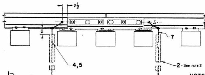
SUPPORTED JOINT
