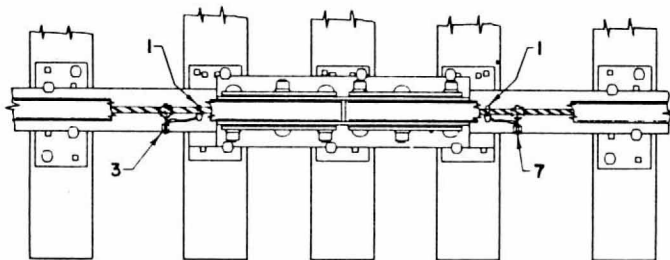
SUPPORTED JOINT
