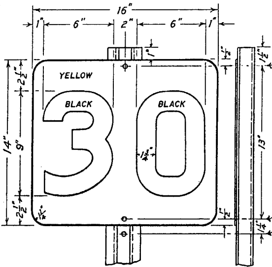
FIG-255 REDUCE SPEED BOARD
