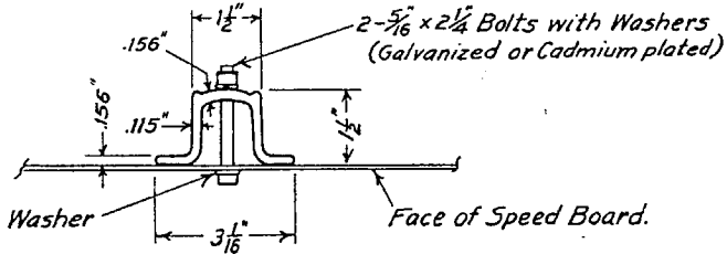
CHANNEL SECTION OF POSTS
