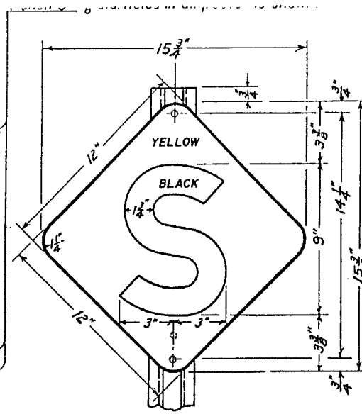
FIG-256 SLOW SPEED BOARD
