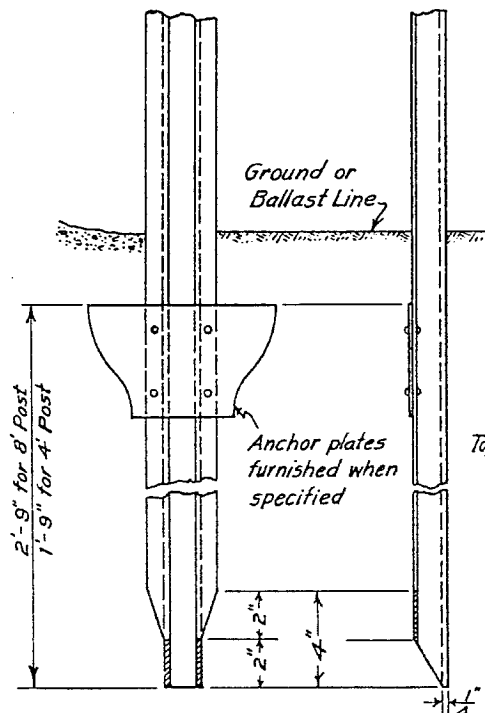
DETAILS OF POSTS
