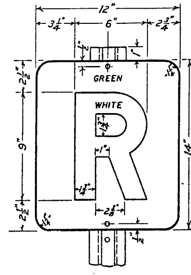
FIG-257 RESUME SPEED BOARD
