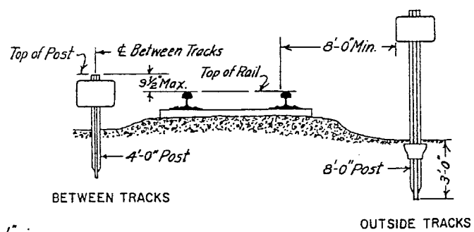
SECTION LOCATION OF SPEED BOARDS
