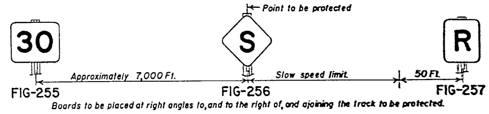
TRACK LOCATION OF SPEED BOARDS
